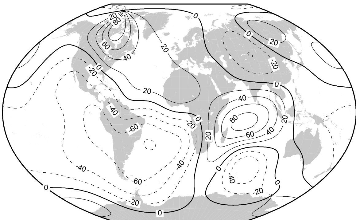
Secular variation of horizontal intensity (nT/yr) for 2005.0-2010.0.
