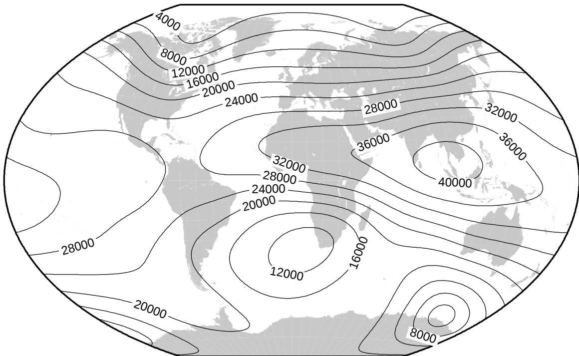
Horizontal intensity (nT) at 2005.0.
