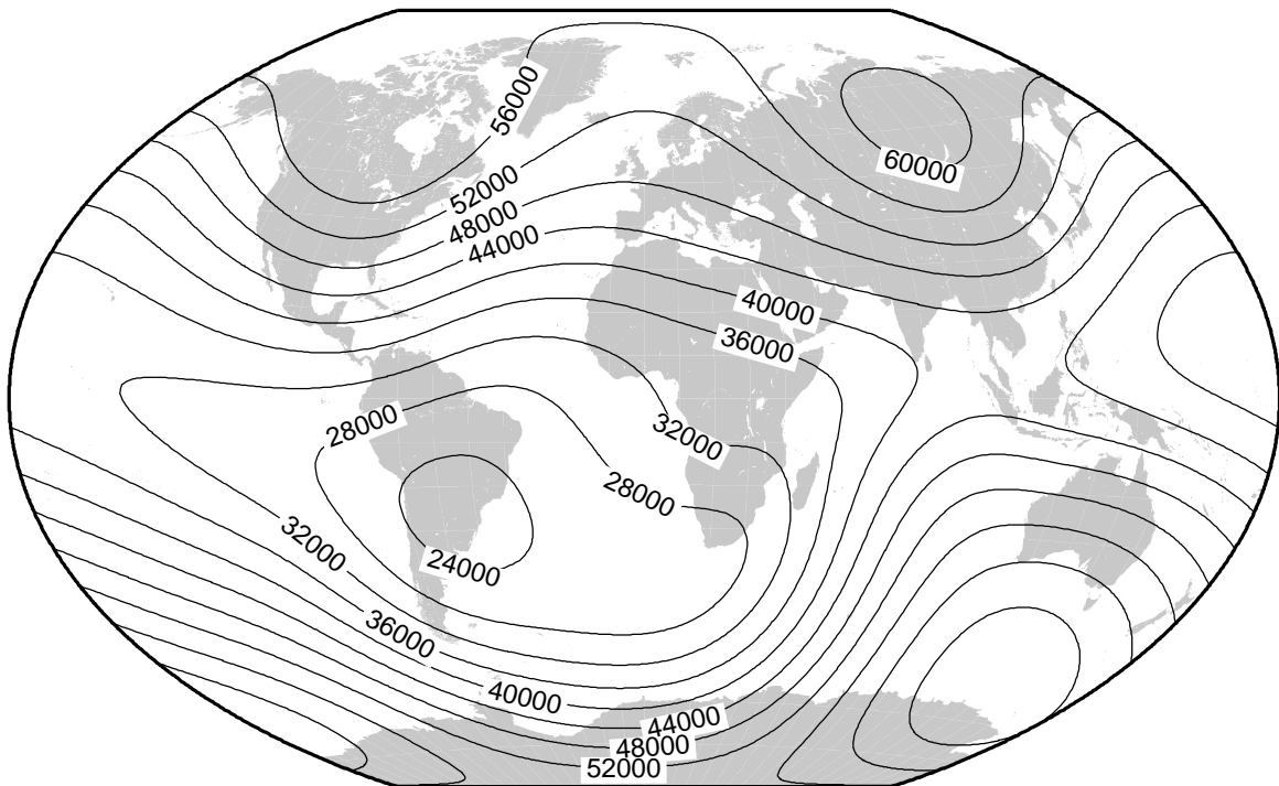
Total intensity (nT) at 2005.0.
