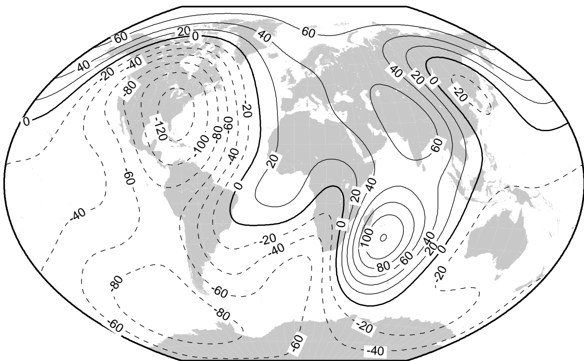
Secular variation of total intensity (nT/yr) for 2005.0-2010.0.
