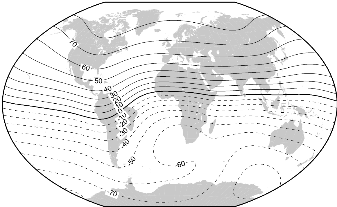
Inclination (degrees) at 2005.0.
