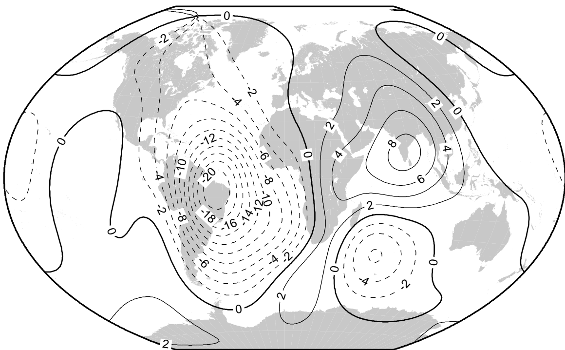
Secular variation of inclination (min/yr) for 2005.0-2010.0.
