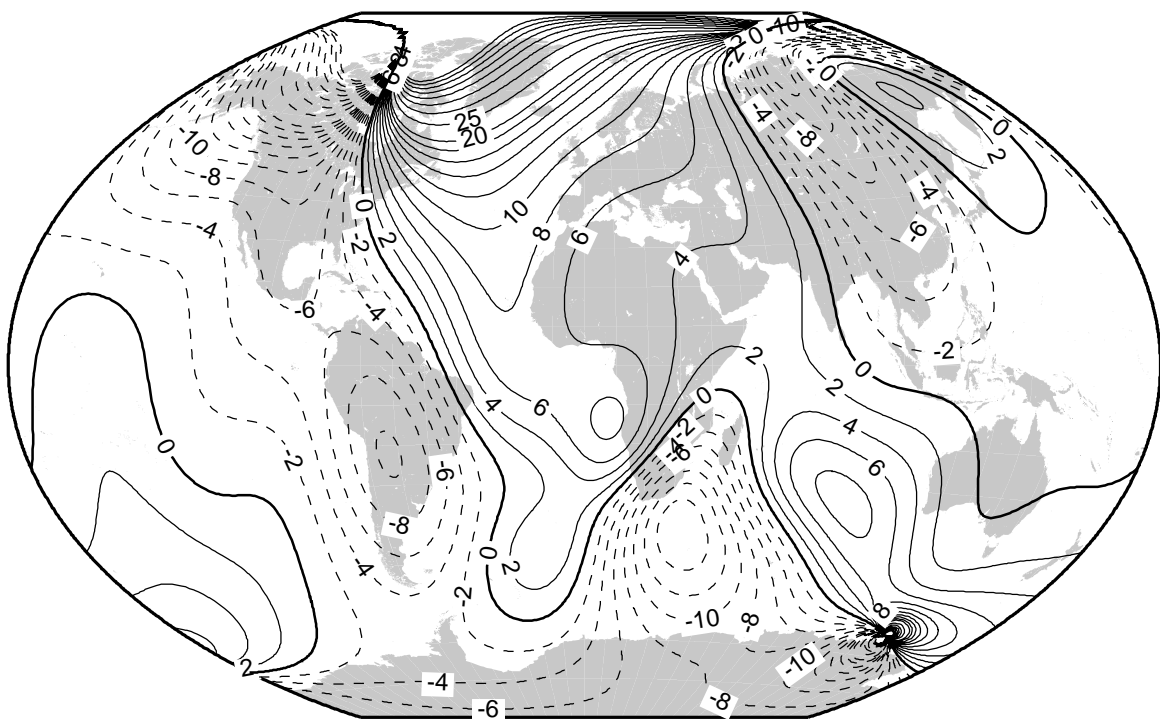
Secular variation of declination (min/yr) for 2005.0-2010.0.
