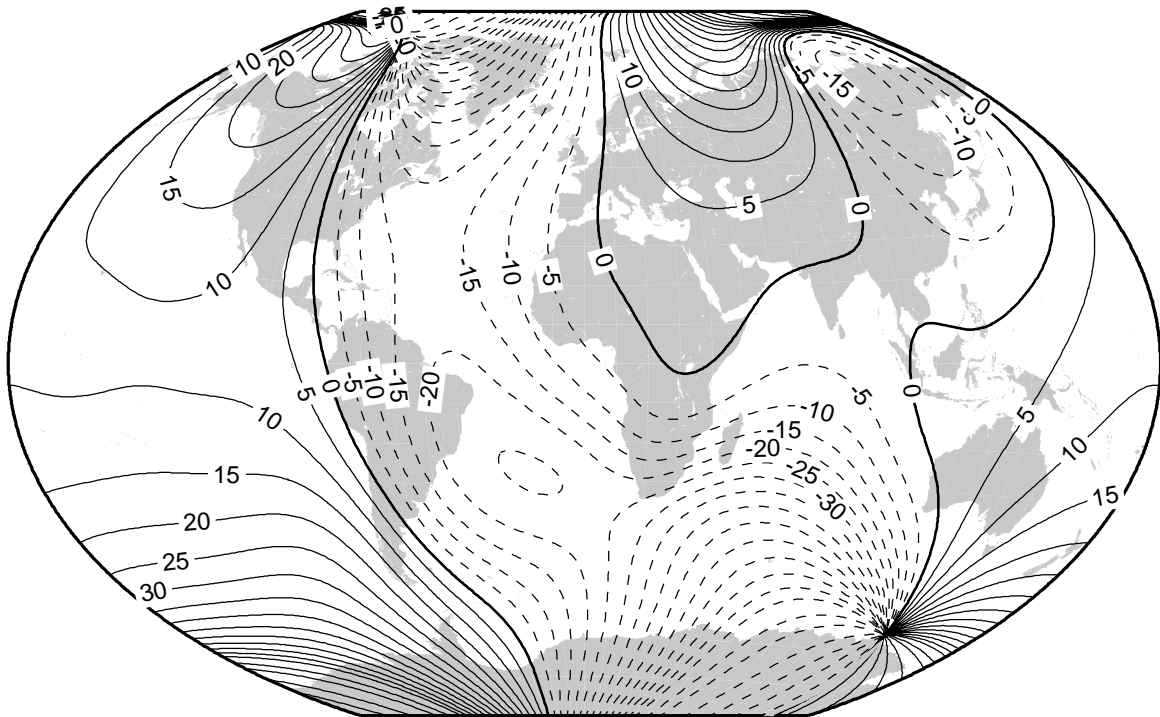
Declination (degrees) at 2005.0.
